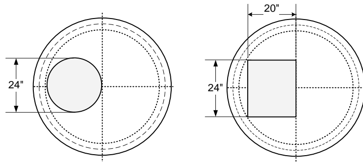
Top Slab Plan View
